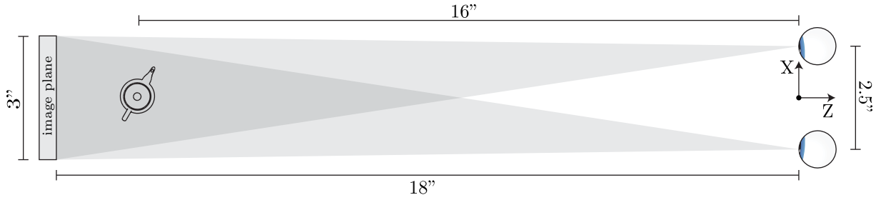
Figure 10: Teapot scene
